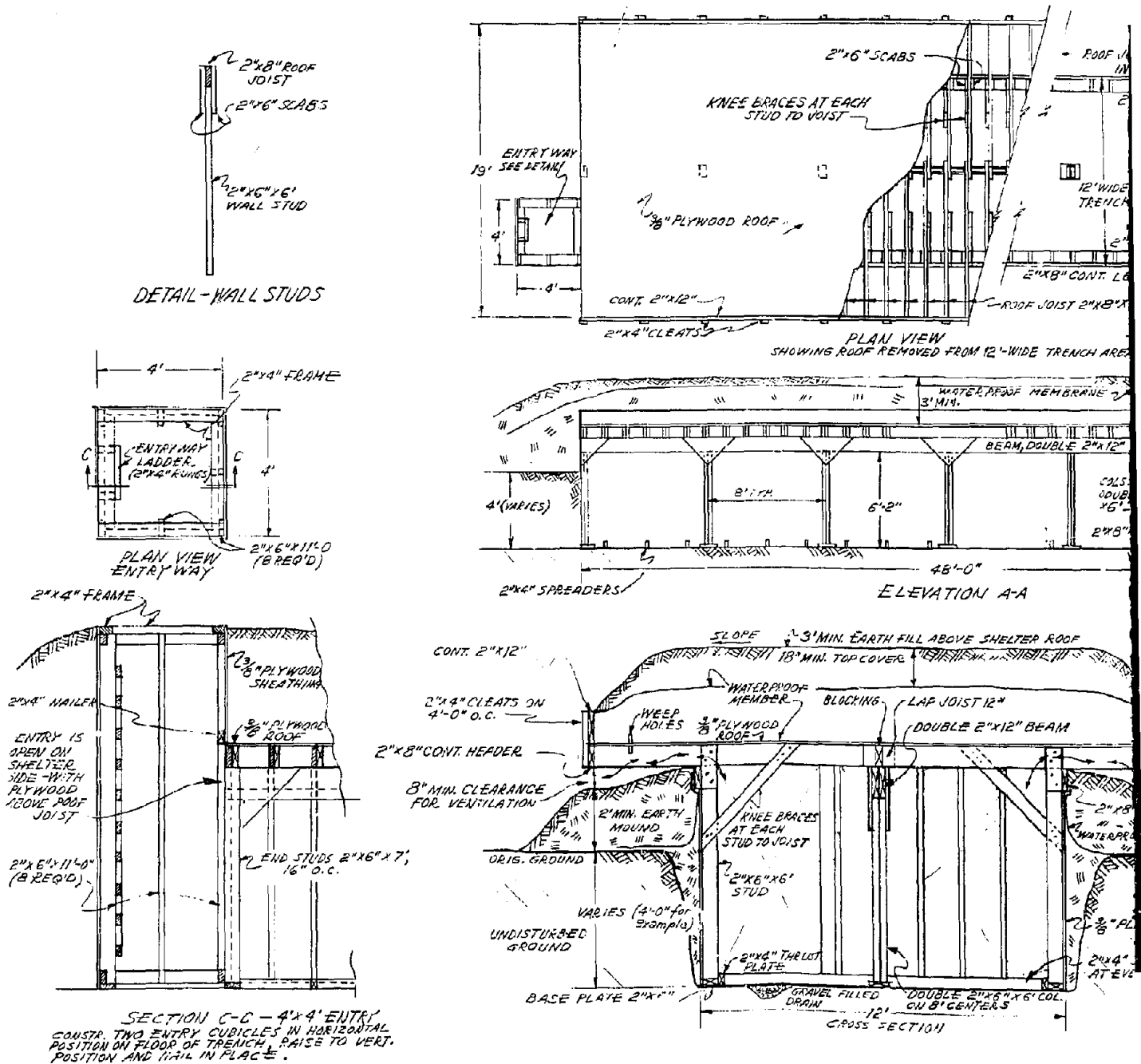
Fig. A-9.2. Rigid-Frame, Continuous Vent, Construction Methods
